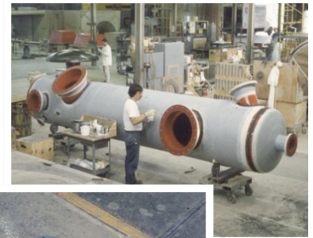
CPVC Lined Scrubber
